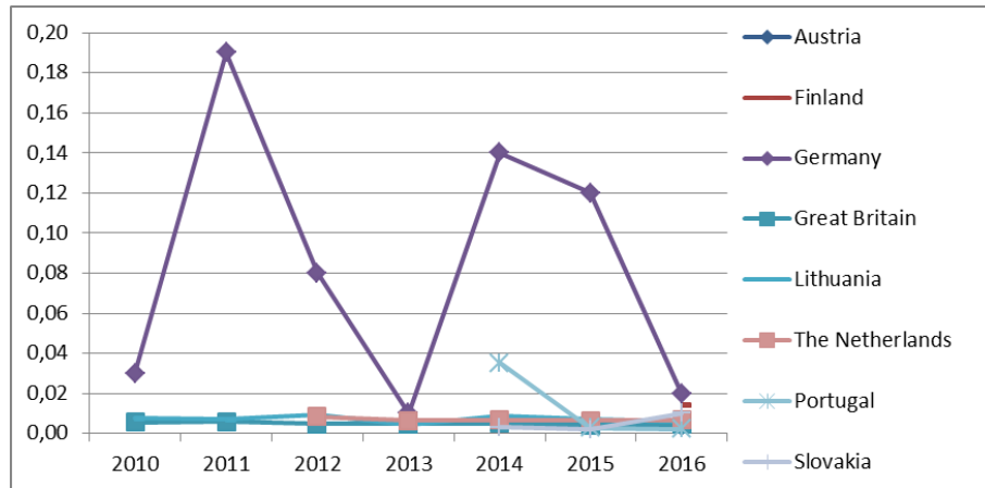
Figure 26 – Gas: unplanned SAIFI (interruptions per customer)
