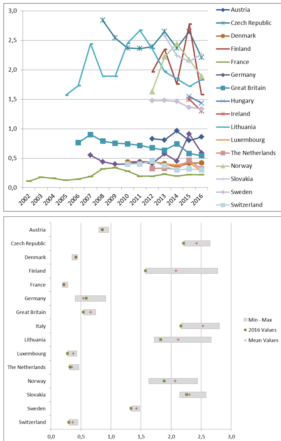
Figure 16 – Electricity: planned and unplanned SAIFI, including exceptional events, only countries not exceeding 3 interruptions
