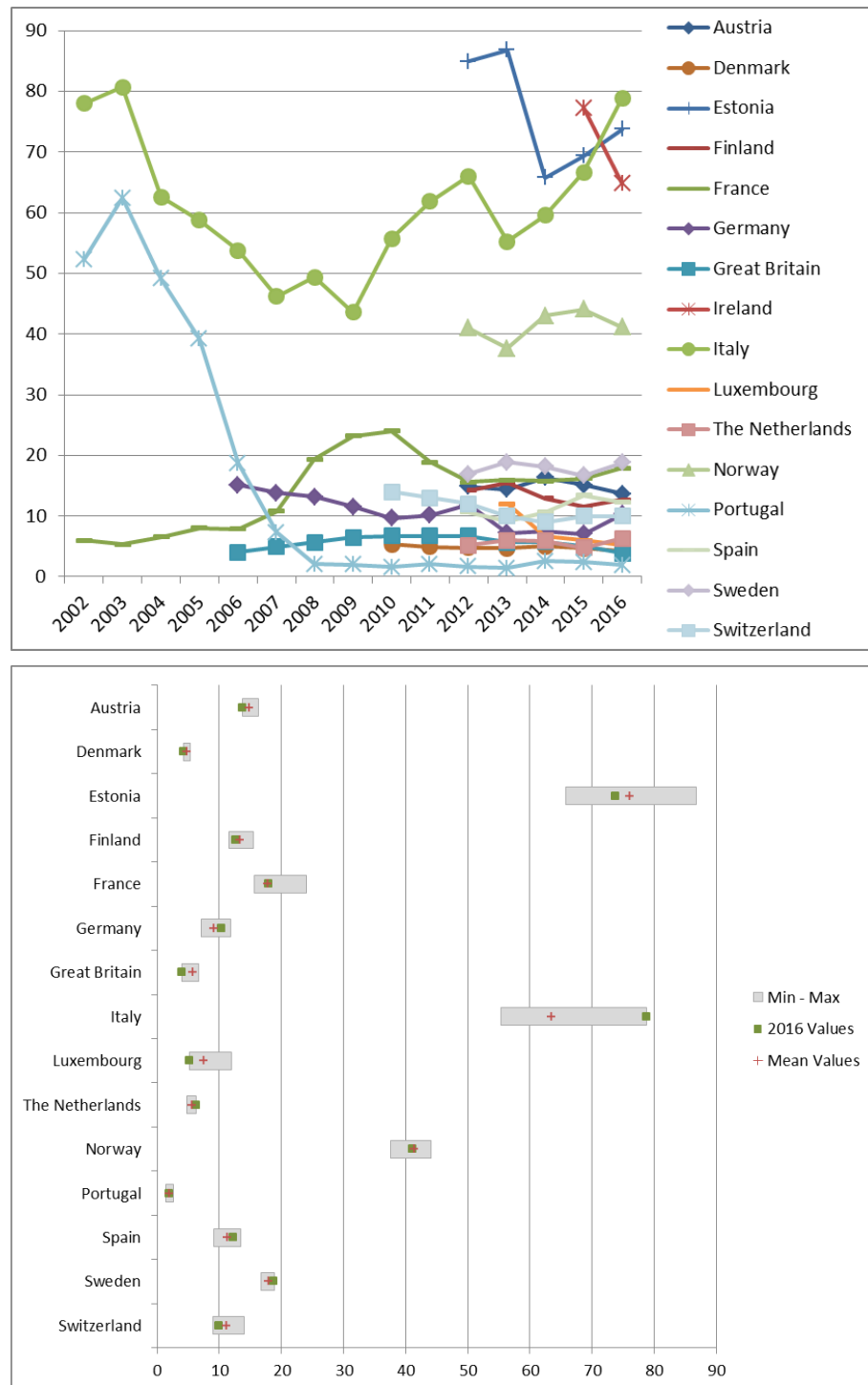
Figure 6 – Electricity: planned SAIDI, only countries not exceeding 100 minutes (minutes per customer) – time series and min-max
